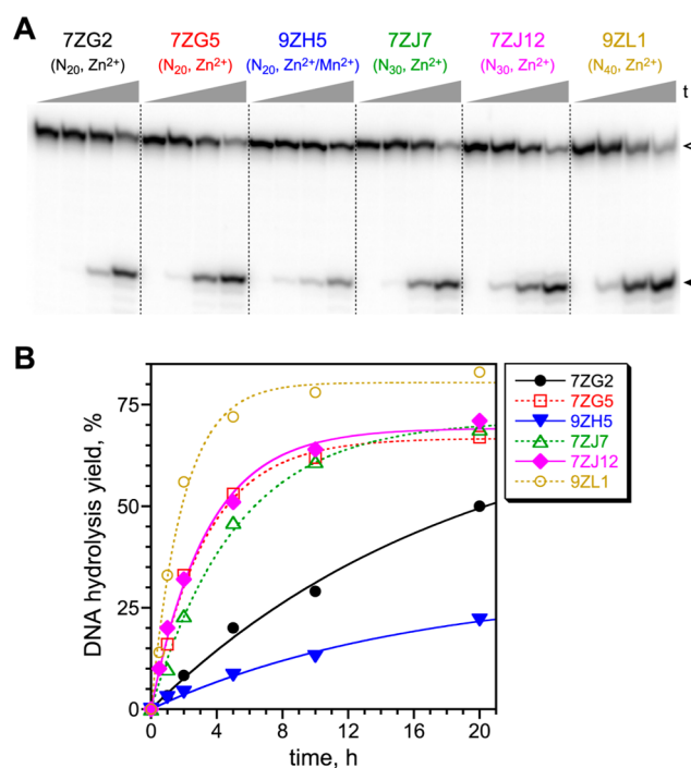
Figure 5. Activities of deoxyribozymes from the follow-up N_{20} , N_{30} , and N_{40} selections for DNA-catalyzed DNA hydrolysis. (A) PAGE image for each of the six new deoxyribozymes, showing representative time points ( t = 30 \text{ s} , 15 \text{ min} , 2 \text{ h} , and 20 \text{ h} ). Substrate (open arrowhead) and product (filled arrowhead) are marked. Incubation conditions: 70 \text{ mM} HEPES, \text{pH } 7.5 , 1 \text{ mM} ZnCl_2 , 20 \text{ mM} MnCl_2 if indicated, and 150 \text{ mM} NaCl at 37 \text{ }^\circ\text{C} . (B) Kinetic plots. k_{obs} values are tabulated in Supporting Information, Table S4.
