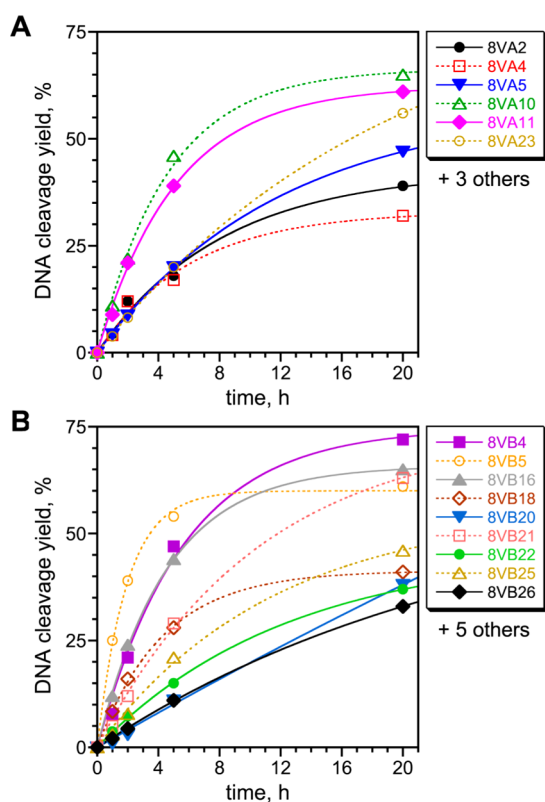
Figure 3. Kinetic plots for individual deoxyribozymes from the (A) N_{20} and (B) N_{30} selections for DNA cleavage. Kinetic plots for several additional deoxyribozymes from each selection experiment are shown in Supporting Information, Figure S2. k_{obs} values are tabulated in Supporting Information, Table S4. Incubation conditions as in Figure 2.
