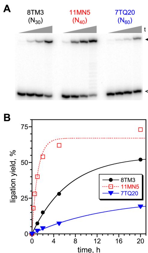
Figure 6. Activities of deoxyribozymes from the selections for DNA-catalyzed nucleopeptide linkage formation. (A) PAGE image showing representative time points ( t = 30 s, 30 min, 2 h, and 20 h). Incubation conditions: 50 mM HEPES, pH 7.5, 20 mM MnCl_2 , 40 mM MgCl_2 , 150 mM NaCl, and 2 mM KCl at 37 °C. Substrate (open arrowhead) and product (filled arrowhead) are marked. For N_{30} , 8TM3 was the only new deoxyribozyme identified, along with two closely related sequence variants. For N_{40} , 11MN5 was the best deoxyribozyme identified previously by direct selection; 31 data shown here were newly acquired for comparison. For N_{60} , 7TQ20 was one of two different deoxyribozymes found, along with six close sequence variants; the other deoxyribozyme, 7TQ46 (no variants found), had slightly lower activity. (B) Kinetic plots. k_{obs} values are tabulated in Supporting Information, Table S4.
