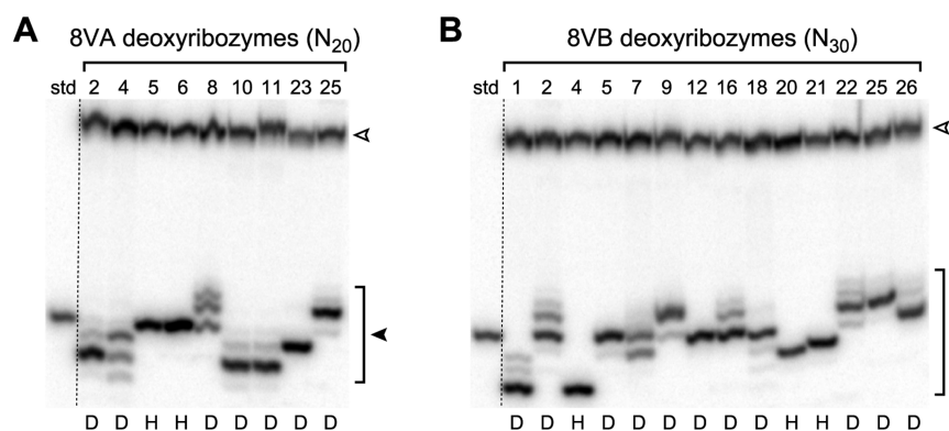
Figure 2. Various substrate cleavage sites for deoxyribozymes from the initial (A) N_{20} and (B) N_{30} selections for DNA-catalyzed DNA cleavage. Individual deoxyribozymes are denoted 8VA followed by a clone number for N_{20} and 8VB followed by a clone number for N_{30} . Each deoxyribozyme was allowed to cleave the 5'- ^{32} P-radiolabeled DNA substrate ( open arrowhead ), resulting in a product band ( filled arrowhead ) whose PAGE migration rate relative to the standard suggests the cleavage site. The standard sample corresponds to hydrolysis of the substrate sequence at the position noted in the Experimental Procedures. Incubation conditions: 70 mM HEPES, pH 7.5, 1 mM ZnCl_2 , 20 mM MnCl_2 , 40 mM MgCl_2 , and 150 mM NaCl at 37 °C ( t = 20 h). Quantification of cleavage kinetics for each deoxyribozyme is provided in Figure 3. The reaction type (i.e., substrate hydrolysis, or substrate deglycosylation followed by two \beta -eliminations) and precise site of each cleavage reaction was assigned with confidence for each deoxyribozyme by MALDI mass spectrometry of the products (Figure 4; see Supporting Information, Tables S1 and S2 for all data values and cleavage-site assignments). The type of reaction catalyzed by each deoxyribozyme is marked below its lane with "H" for hydrolysis or "D" for deglycosylation.
