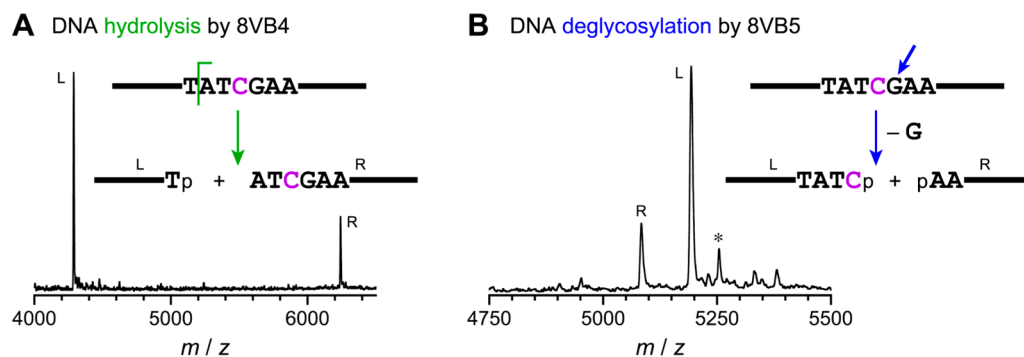
Figure 4. Representative MALDI mass spectra to assign cleavage reactions and sites for deoxyribozymes from the initial N_{20} and N_{30} selections for DNA cleavage. All mass spectra data and precise cleavage-site assignments are tabulated in Supporting Information, Tables S1 and S2. The indicated C nucleotide of the substrate was not base-paired with either deoxyribozyme binding arm (see Figure 1). (A) 8VB4 deoxyribozyme, which hydrolyzes the DNA substrate at a specific phosphodiester linkage and forms 3'-phosphate and 5'-hydroxyl products. Some of the new DNA-hydrolyzing deoxyribozymes lead instead to 3'-hydroxyl and 5'-phosphate products. (B) 8VB5 deoxyribozyme, which deglycosylates the DNA substrate at a specific guanosine. After two subsequent \beta -elimination reactions, the products are missing the entire G nucleoside and have 3'-phosphate and 5'-phosphate groups. Some of the new DNA-deglycosylating deoxyribozymes are not site-specific and deglycosylate the substrate at either of two adjacent nucleotide positions. In the spectrum of panel B, the asterisk denotes the peak for uncleaved substrate with z = 2 .
