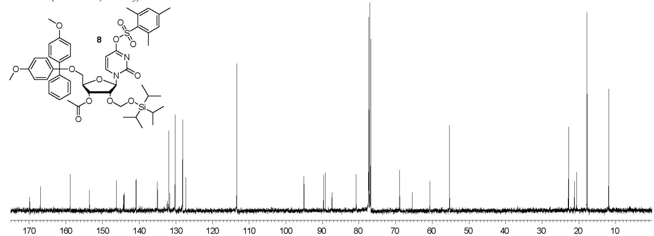
13 C NMR (125 MHz, CDCl 3 ) of 8 .
