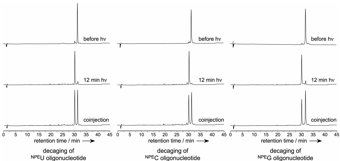
Figure S1. HPLC traces analogous to that shown in Figure 2b for decaging of three NPE-caged oligonucleotides (photolysis with 300-W Xe arc lamp).
