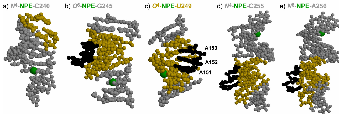
Figure S7. Structural context of caging sites for nucleotide positions in the lower portion of P4-P6, within or near the tetraloop receptor (gold; nucleotides 222–227 and 247–251). Adenosine nucleotides of the tetraloop are black (A151–A153). Other nucleotides of P4-P6 are grey. In all of these cases, only small effects due to NPE-caging of the indicated nucleobase were observed by native PAGE (Figure 4 and Figure S9).
