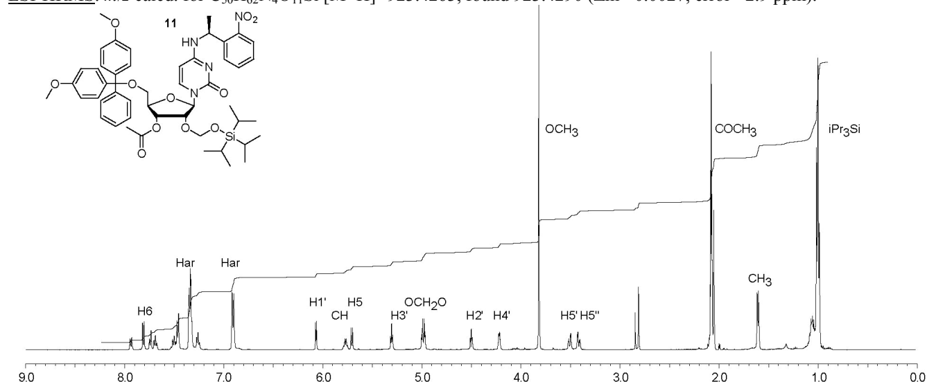
1 H NMR (500 MHz, acetone- d 6 ) of 11 .
