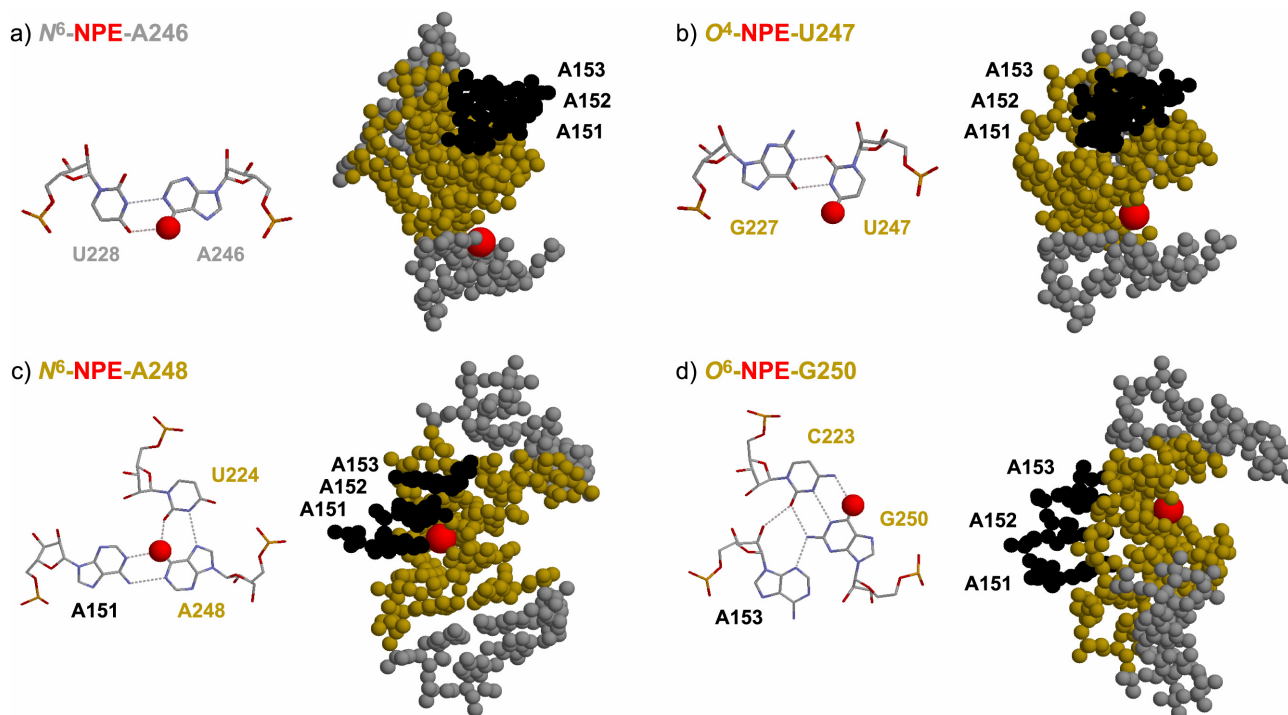
Figure S6. Structural context of caging sites for the four P4-P6 nucleotide positions for which unambiguous structural disruptions were observed by native PAGE (Figure 4b, red). All four sites are located within or near the tetraloop receptor. Images were rendered in RasMol using coordinates from the X-ray structure. [2] As in Figure 3, the adenosine nucleotides of the tetraloop are colored black (A151–A153); the receptor nucleotides are gold (222–227 and 247–251); and other P4-P6 nucleotides are grey (220–221, 228–229, 245–246, and 252–253). For N 6 -NPE-A248 (panel c), the caging site is buried within the tetraloop-receptor interface; therefore, appending the NPE group should introduce severe steric clashes as well as disrupt several hydrogen bonds. For the other three nucleotides (panels a, b, and d), the NPE group should disrupt at least one tertiary hydrogen bond, whereas there appears to be sufficient space to accommodate the NPE group in terms of its steric interactions. In all cases, the effects of caging upon stacking interactions are difficult to predict from these molecular models.
