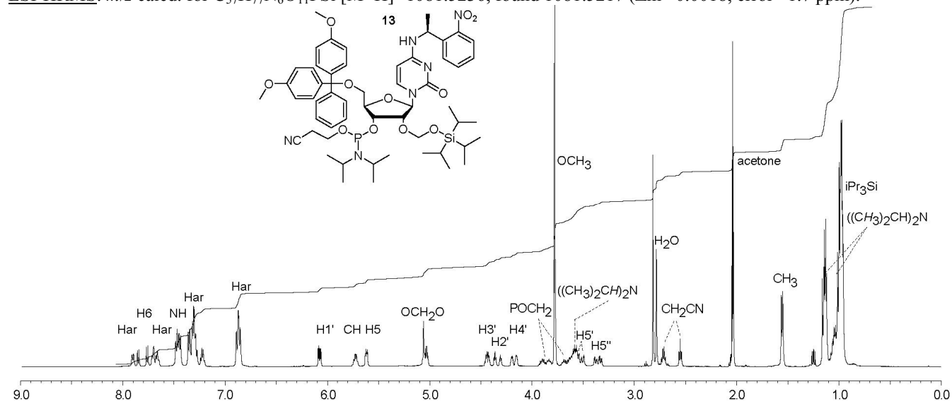
1 H NMR (500 MHz, acetone- d 6 ) of 13 .
