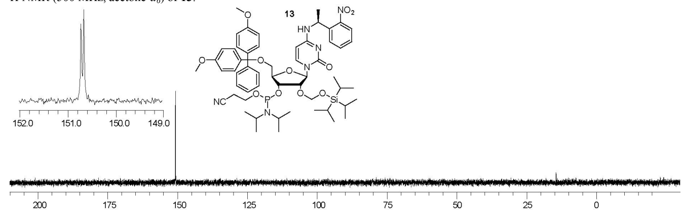
31 P NMR (202 MHz, acetone- d 6 ) of 13 .
