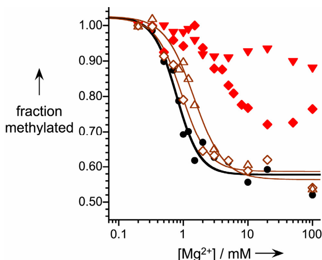
Figure S10. DMS probing experiments with caged P4-P6 RNAs before and after photolysis to remove the caging group. The U247 ( \blacklozenge ) and G250 ( \blacktriangledown ) NPE-caged P4-P6 derivatives were examined by DMS probing before and after 10 min photolysis with the arc lamp as described on page S3. Closed symbols ( red ) are before photolysis, and open symbols ( brown ) are after photolysis. Wild-type P4-P6 RNA ( \bullet ) was also examined.
