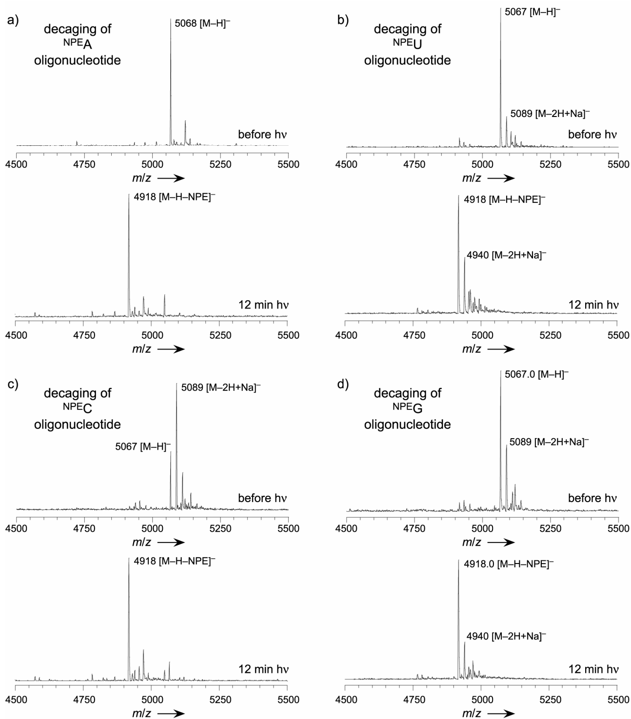
Figure S2. ESI-MS data that demonstrate decaging of the four NPE-caged oligonucleotides. Photolysis used the 300-W Xe arc lamp. The calculated [M-H]^- m/z values for the caged and uncaged 15-mer oligonucleotides are 5066.2 and 4917.1, respectively.
