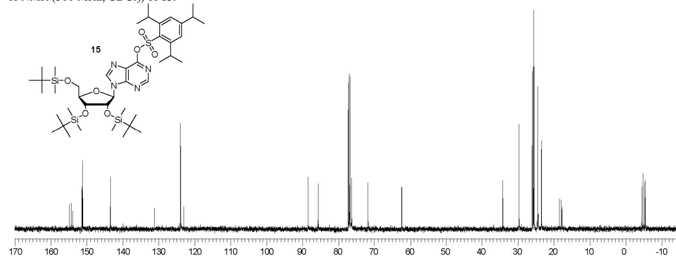
13 C NMR (125 MHz, CDCl 3 ) of 15 .
