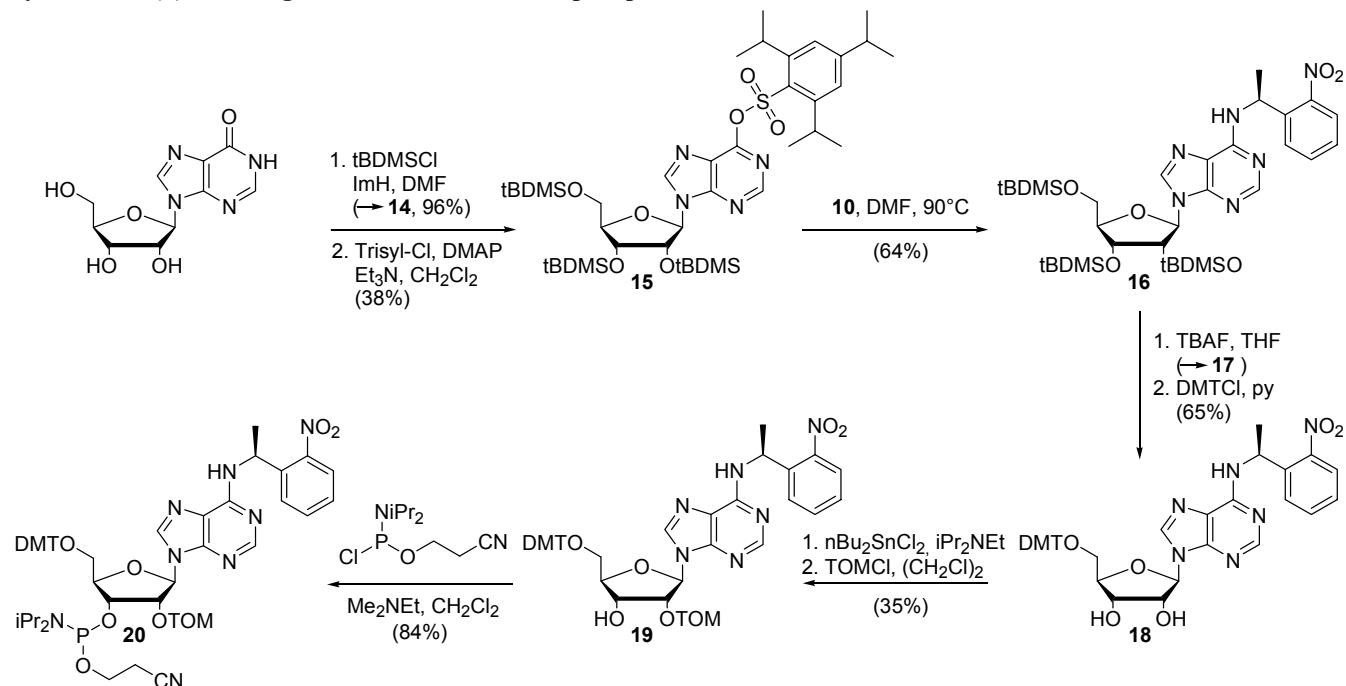
Scheme S2. Synthesis of N 6 -NPE-adenosine phosphoramidite 20 .
