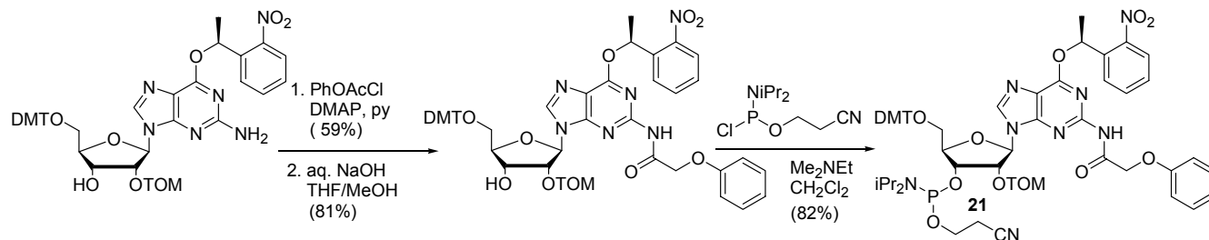
Scheme S3. Synthesis of O 6 -( S )-NPE-guanosine phosphoramidite 21 .
