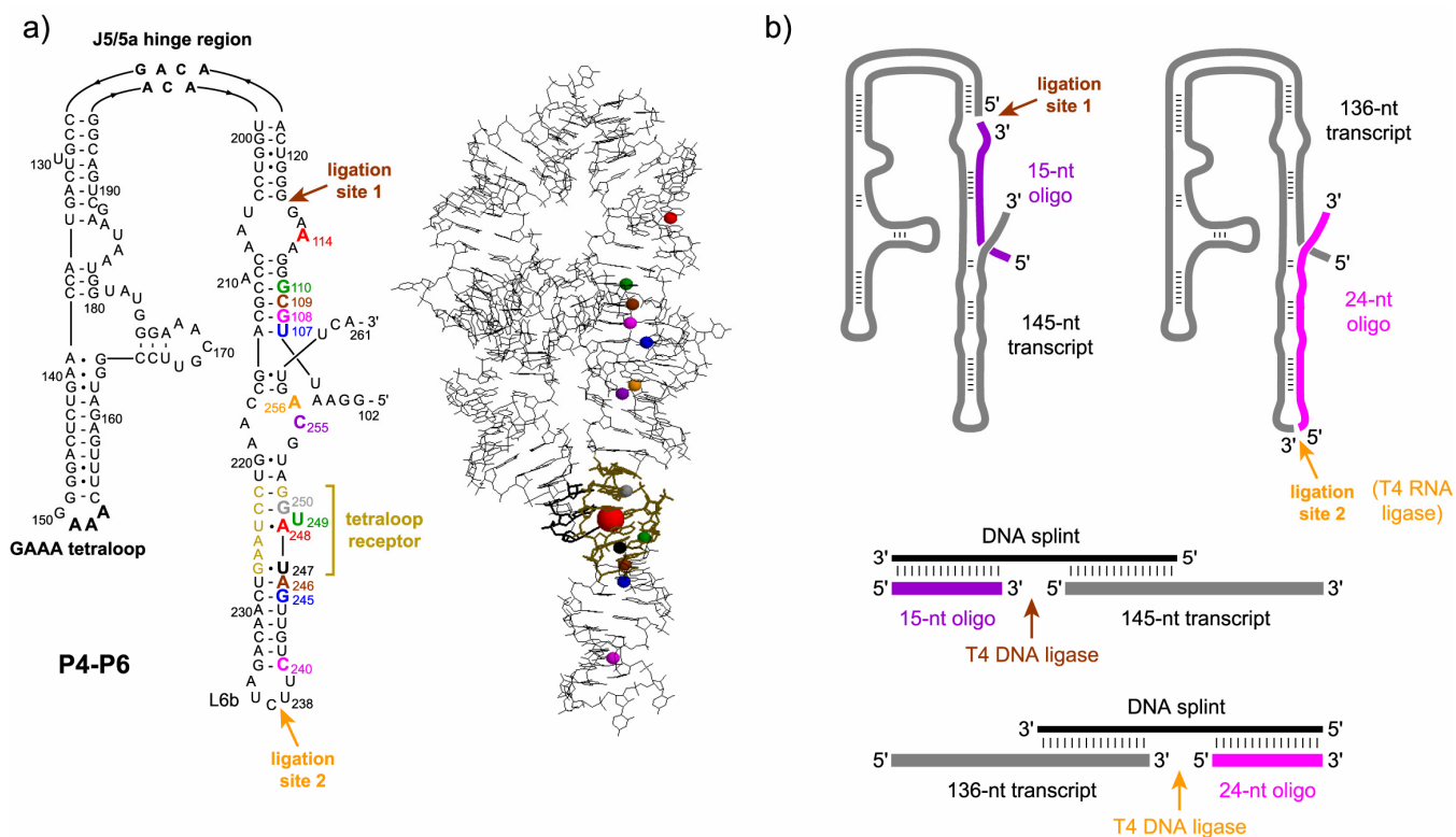
Figure S5. Secondary structure and synthetic strategies to prepare P4-P6 by ligation. a) Secondary structure of P4-P6 with caging sites highlighted. The adjacent tertiary structure is shown in the same orientation as in Figure 3a. b) Ligation strategies. For ligation at site 1, the splint ligation strategy was used (T4 DNA ligase). For ligation at site 2, either an analogous splint ligation strategy was used (T4 DNA ligase), or ligation without a splint was performed (T4 RNA ligase). In the latter case, the secondary structure of P4-P6 itself holds the two RNA partners together.
