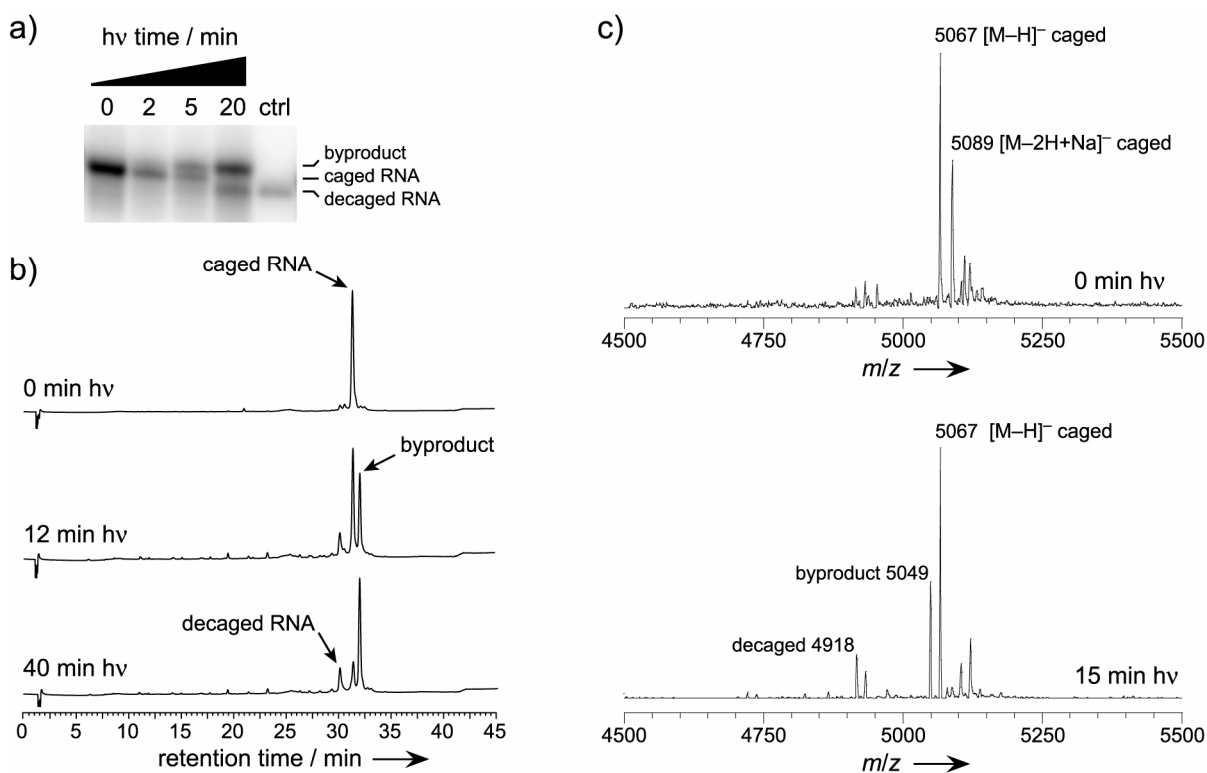
Figure S3. Decaging of the 15-mer RNA oligonucleotide with N^3 -NPE-caged uridine. The caging group was at the same nucleotide position (analogous to U107) as for the O^4 -NPE-caged uridine described on page S3. a) 20% PAGE. Photolysis used a 300-W Xe arc lamp filtered to provide 300-400 nm light. The sample was in 50 mM triethylammonium acetate, pH 7.0. Using a handheld UV lamp (365 nm), photolysis was complete in <60 min, and approximately equal amounts of the decaged RNA and the byproduct were observed (data not shown). b) HPLC traces for photolysis using the arc lamp. The assignment of the HPLC peak for decaged RNA is based on the data shown in Figure S1. c) ESI-MS data for the N^3 -NPE-caged uridine RNA before and after 15 min photolysis with the arc lamp.
