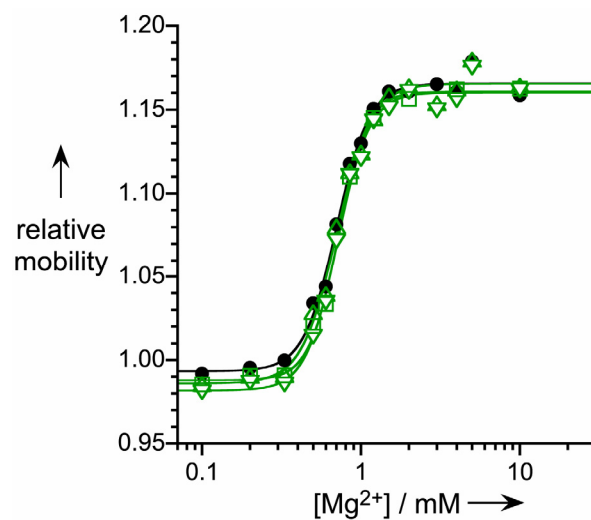
Figure S9. Native PAGE titration data for the NPE-caged G108, G245, and C255 P4-P6 derivatives not shown in Figure 4. In all three cases, the thermodynamic effect due to the caging group was very small.
