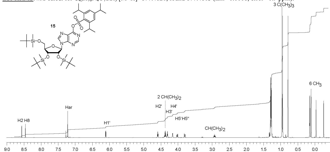
1 H NMR (500 MHz, CDCl 3 ) of 15 .
