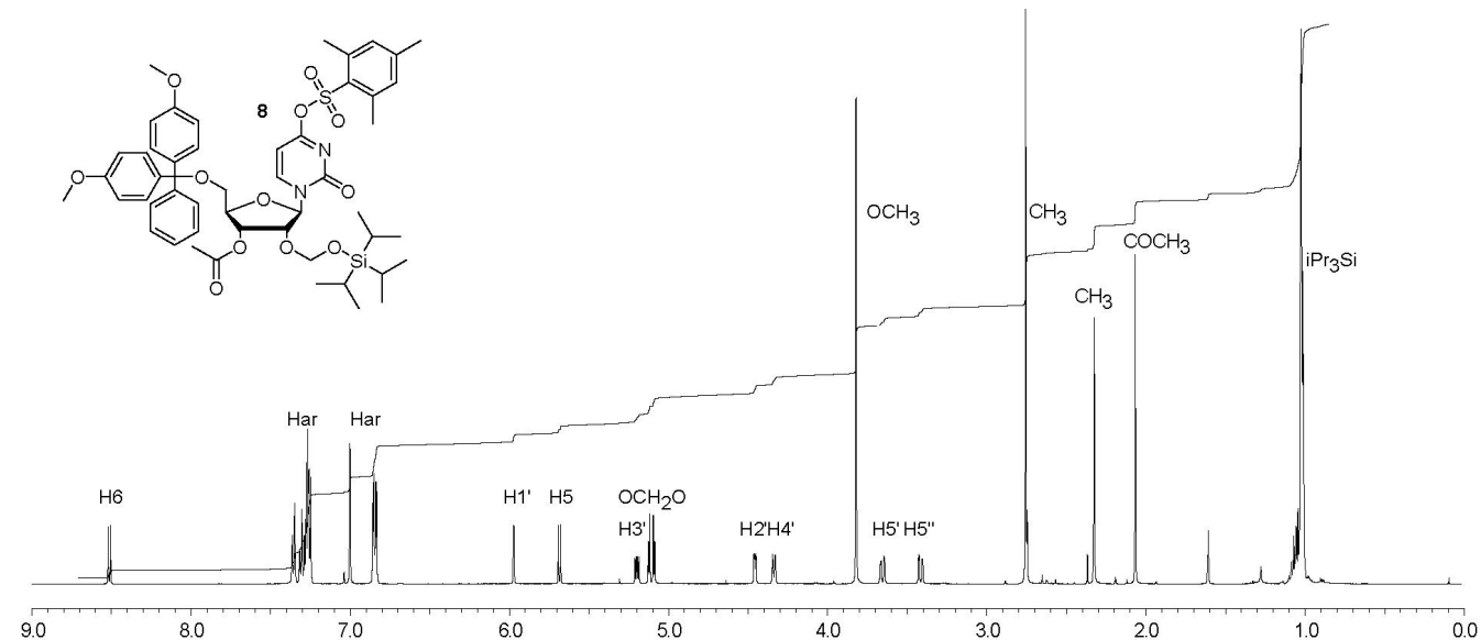
1 H NMR (500 MHz, CDCl 3 ) of 8 .
