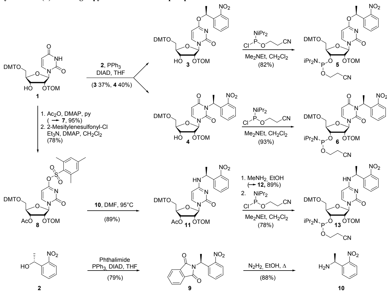
Scheme S1. Syntheses of ( S )-NPE-caged pyrimidine nucleoside phosphoramidites 5 , 6 , and 13 and ( S )-1-(2-nitrophenyl)ethylamine 10 .
