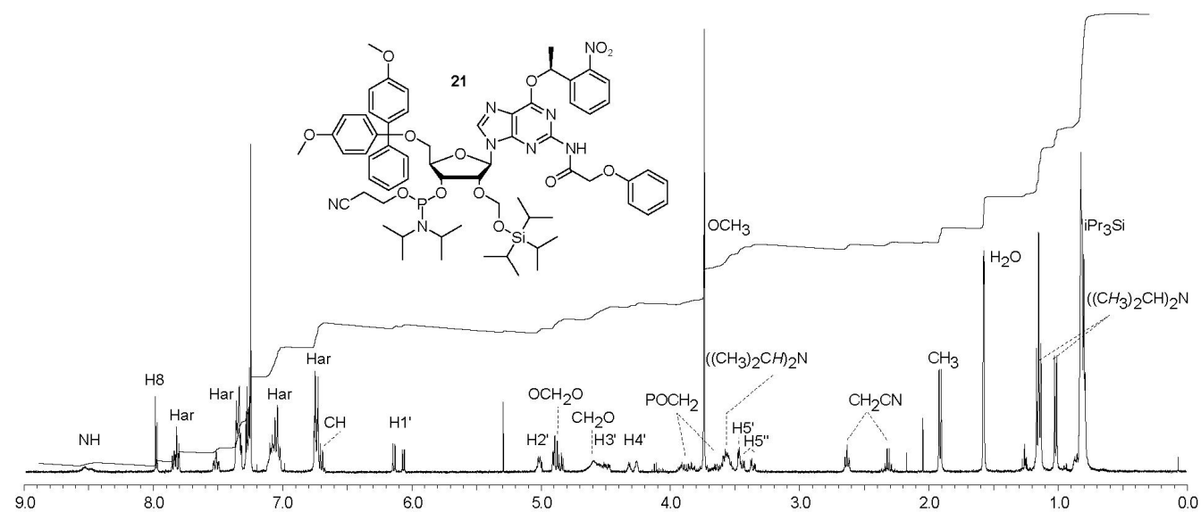
1 H NMR (400 MHz, CDCl 3 ) of 21 .
