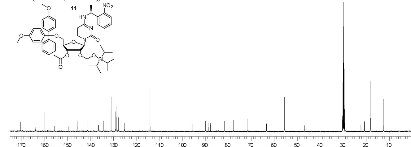
13 C NMR (125 MHz, acetone- d 6 ) of 11 .
