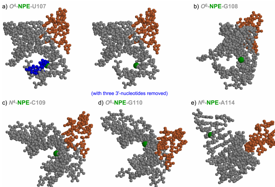
Figure S8. Structural context of caging sites for nucleotide positions in the upper portion of P4-P6, far from the tetraloop-receptor tertiary interaction. Nucleotides 182–188 of the A-rich bulge are colored brown; other P4-P6 nucleotides are grey (105–117, 204–216, and 257–261). In all of these cases, only small effects due to NPE-caging of the indicated nucleobase were observed by native PAGE (Figure 4 and Figure S9). In panel a for the NPE-caged U107 derivative, the three nucleotides U259–A261 at the 3'-end of the P4-P6 molecule are colored blue instead of grey. When these three nucleotides are removed from the model (right structure within panel), the site of caging is accessible to derivatization with a bulky group without appearing to induce a steric clash. It is likely that these three terminal nucleotides of P4-P6 can adopt a conformation other than that observed in the crystal structure without inducing a substantial thermodynamic penalty.
